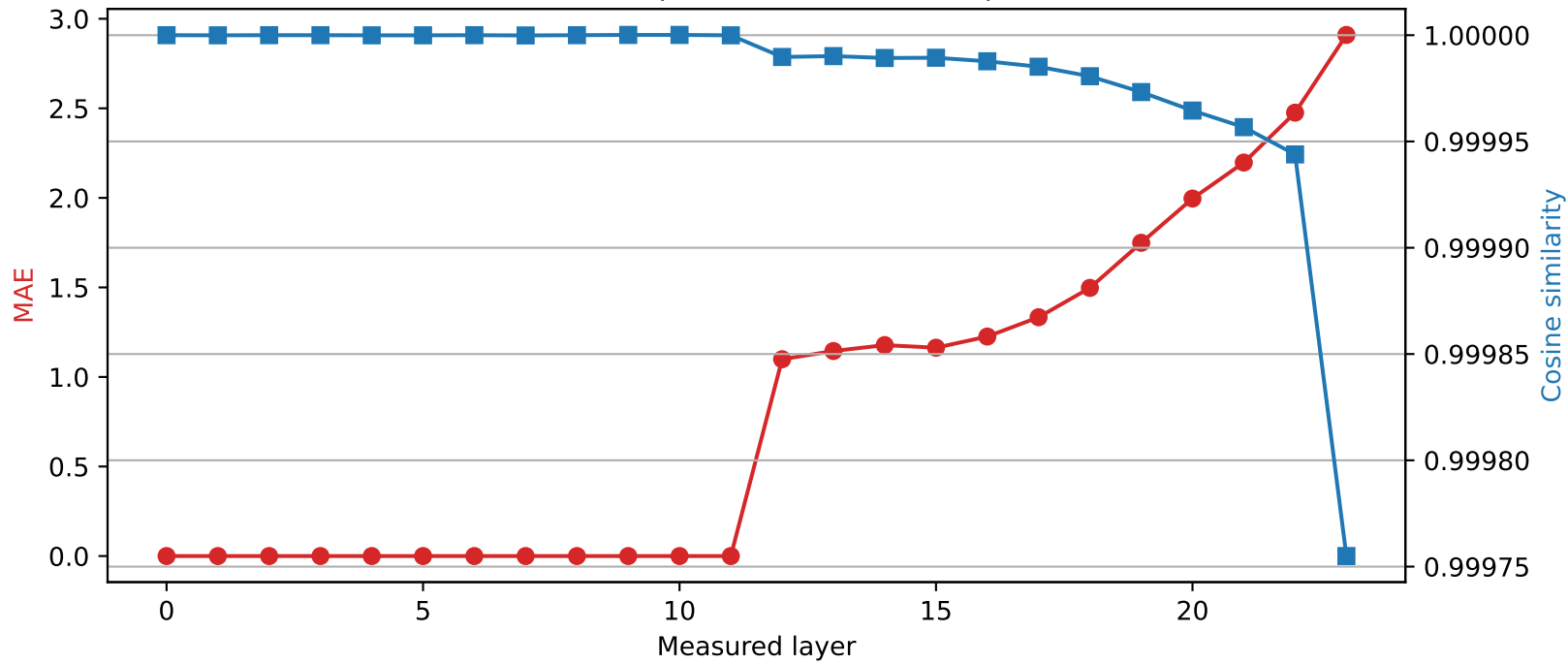
SmolLM2-1.7B-Instruct | Quantized layer 11 | float16 \rightarrow int4
