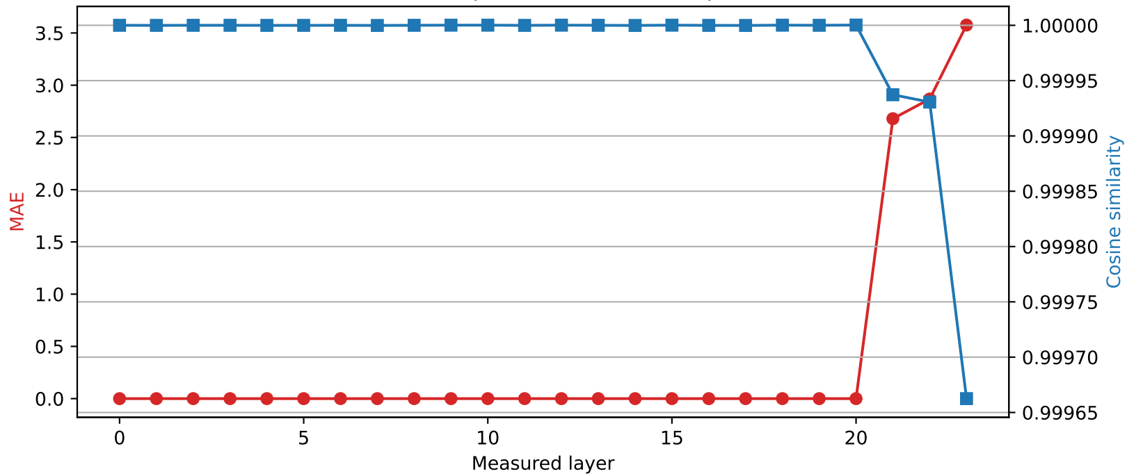
SmolLM2-1.7B-Instruct | Quantized layer 20 | float16 \rightarrow int4
