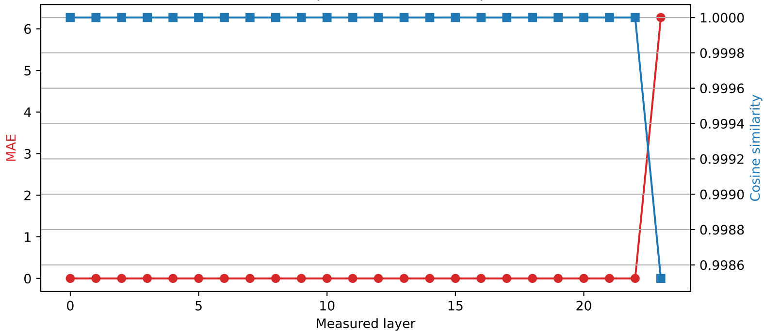
SmolLM2-1.7B-Instruct | Quantized layer 22 | float16 → int4
