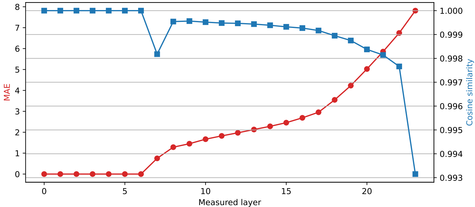
SmolLM2-1.7B-Instruct | Quantized layer 6 | float16 → int4
