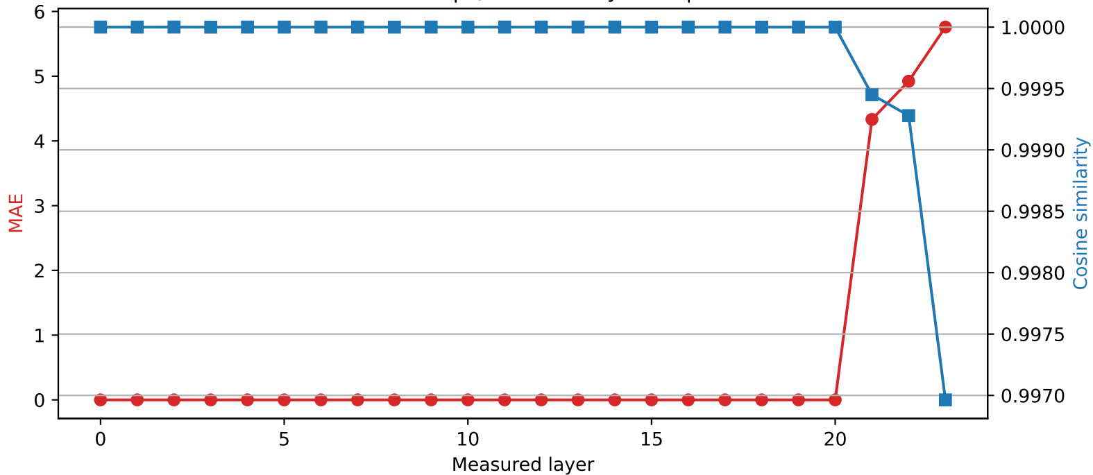
SmolLM2-1.7B-Instruct | Quantized layer 20 | float16 → int4
