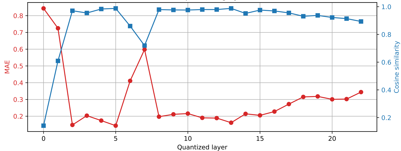
SmolLM2-1.7B-Instruct | Prompt 2 Final RMSNorm output damage | float16 \rightarrow int4
