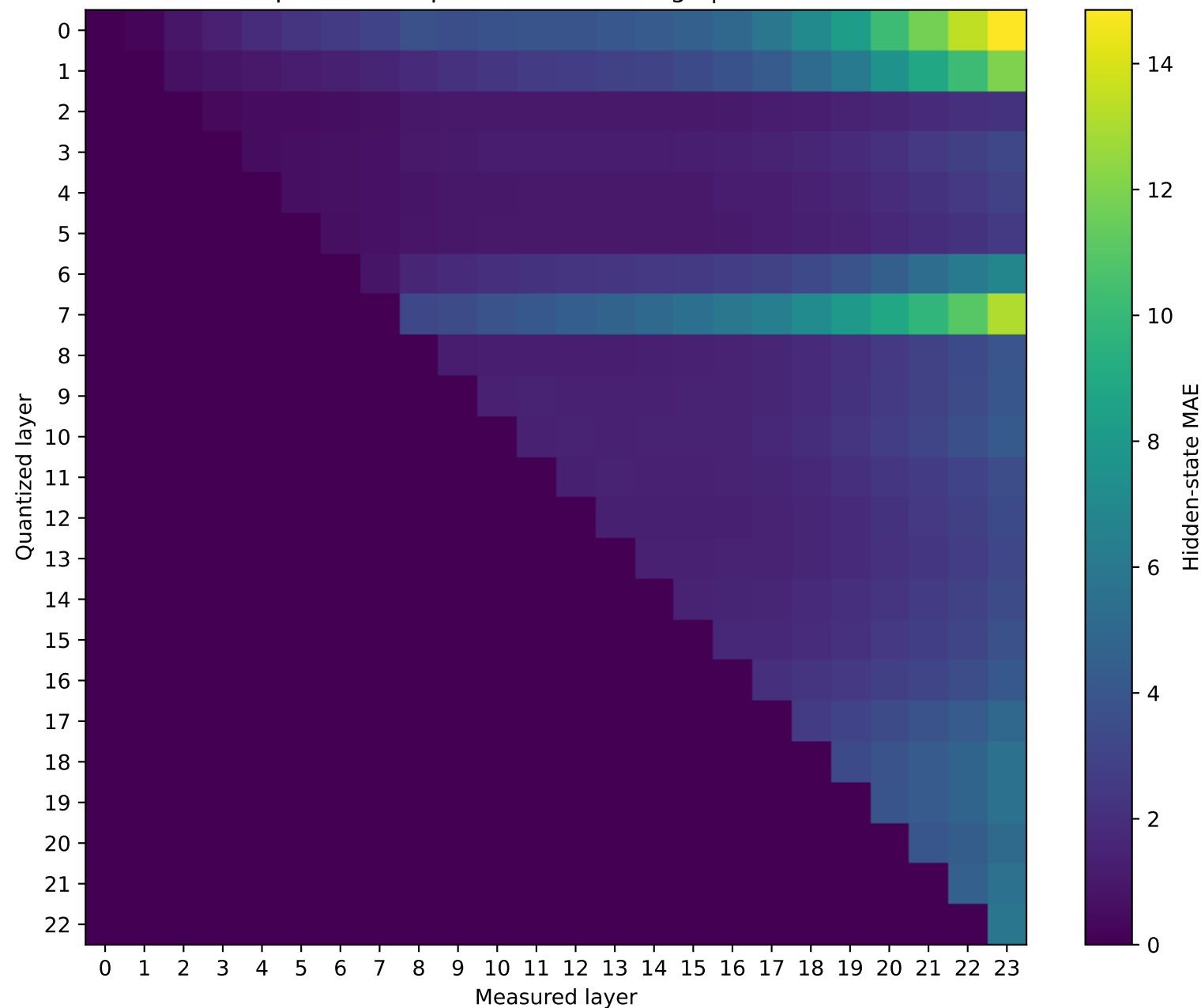
SmolLM2-1.7B-Instruct Prompt 2: MAE representation damage | float16 → int4
