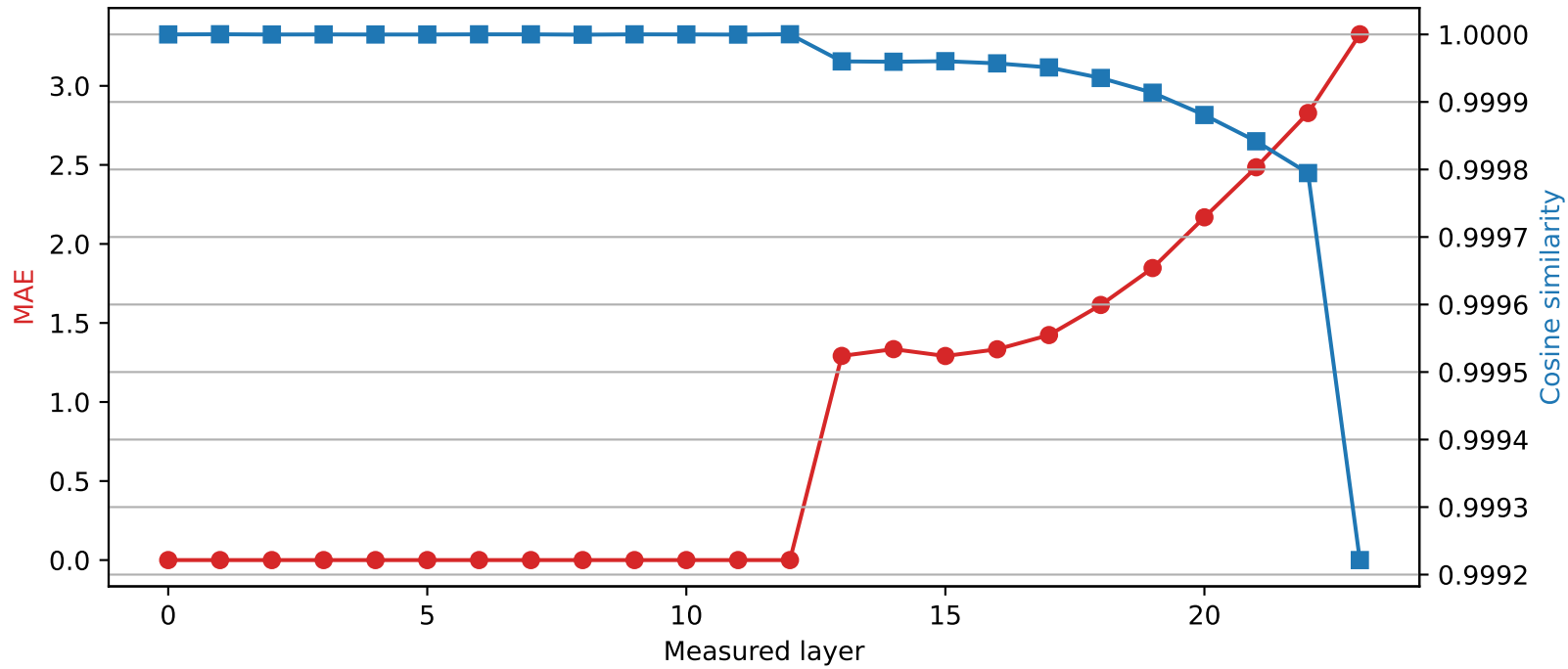
SmolLM2-1.7B-Instruct | Quantized layer 12 | float16 → int4
