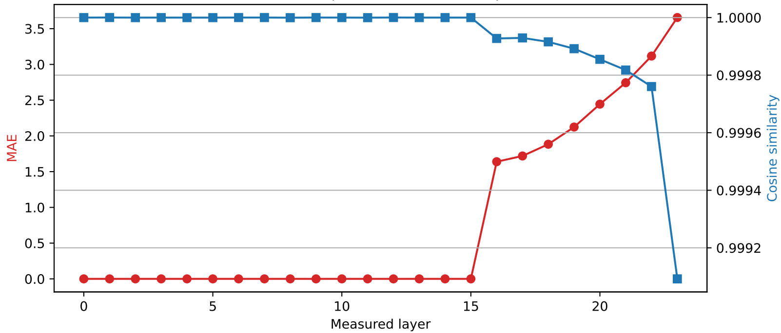
SmolLM2-1.7B-Instruct | Quantized layer 15 | float16 → int4
