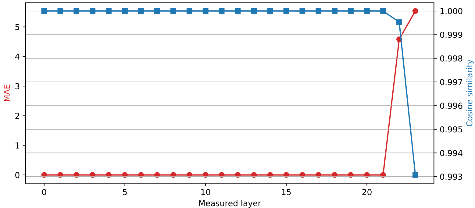
SmolLM2-1.7B-Instruct | Quantized layer 21 | float16 \rightarrow int4
