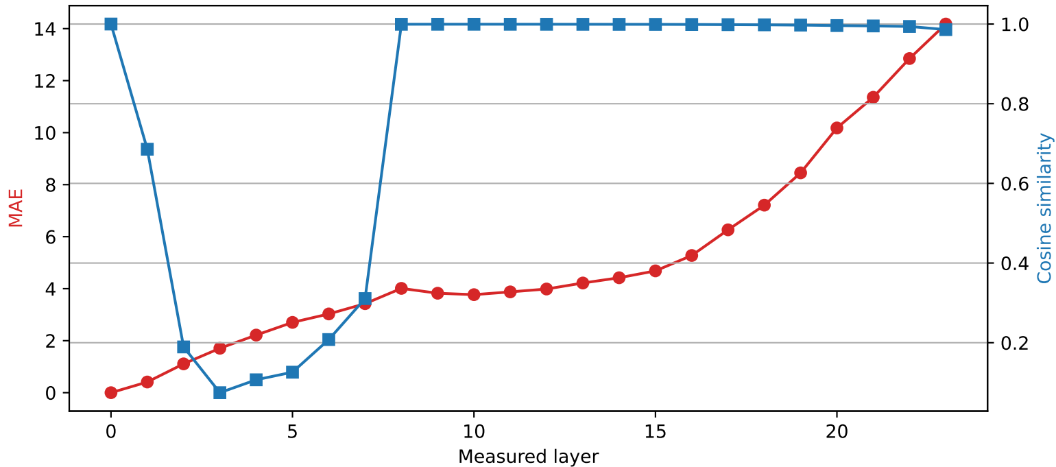
SmolLM2-1.7B-Instruct | Quantized layer 0 | float16 \rightarrow int4
