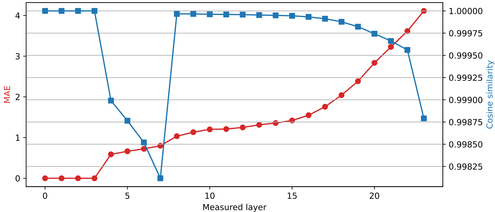
SmolLM2-1.7B-Instruct | Quantized layer 3 | float16 → int4
