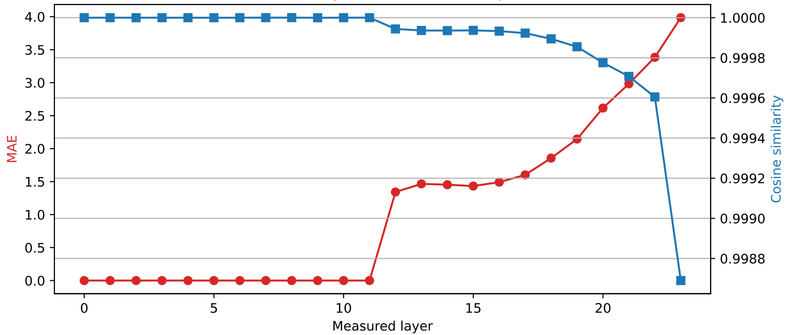
SmolLM2-1.7B-Instruct | Quantized layer 11 | float16 → int4
