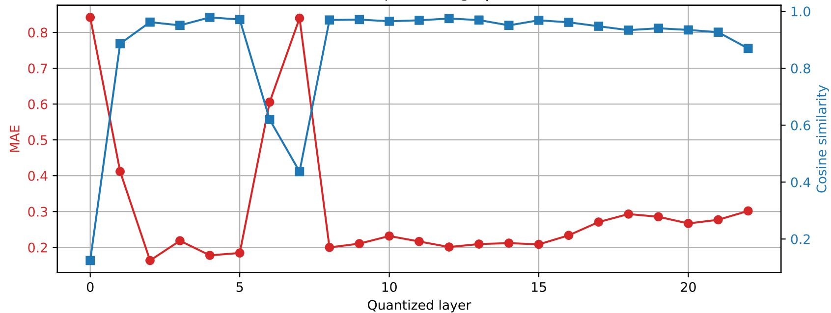
SmolLM2-1.7B-Instruct | Prompt 4 Final RMSNorm output damage | float16 \rightarrow int4
