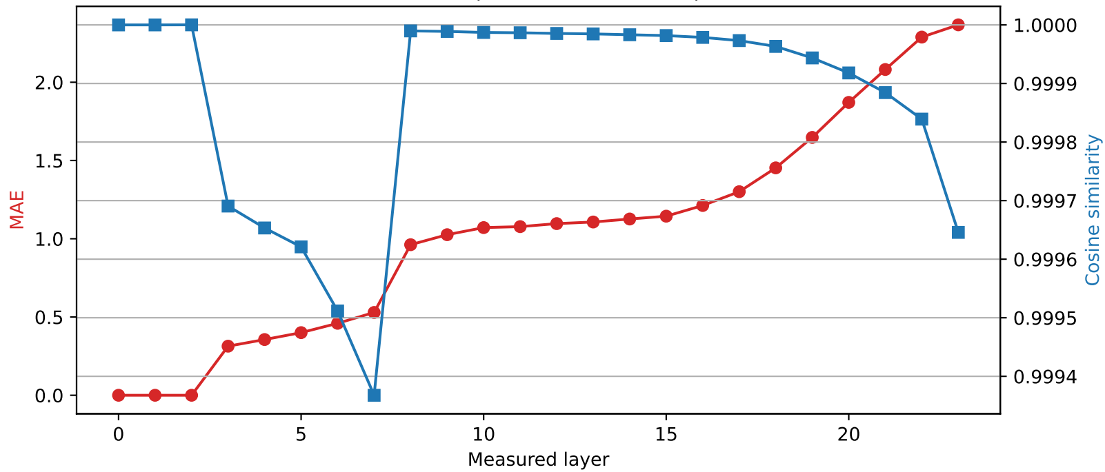
SmolLM2-1.7B-Instruct | Quantized layer 2 | float16 → int4
