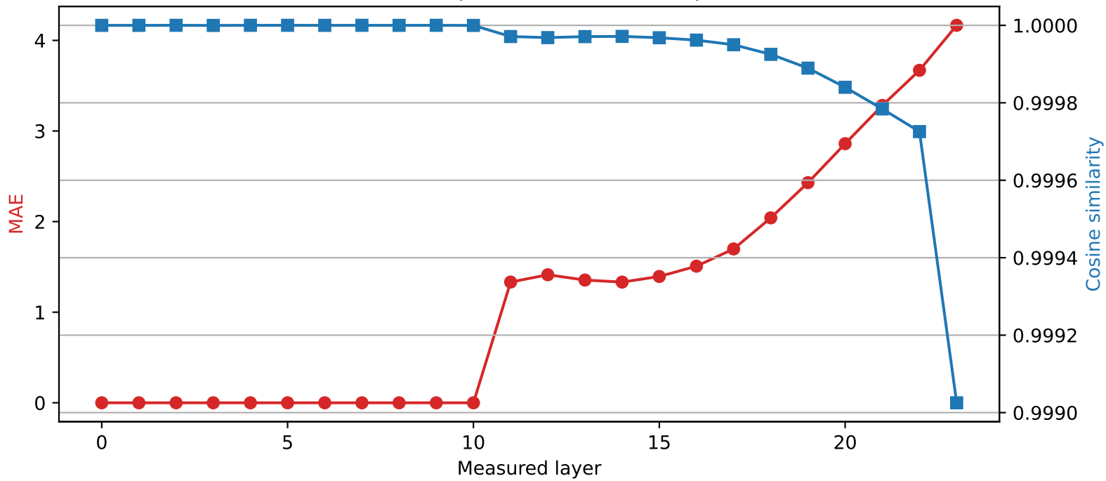
SmolLM2-1.7B-Instruct | Quantized layer 10 | float16 → int4
