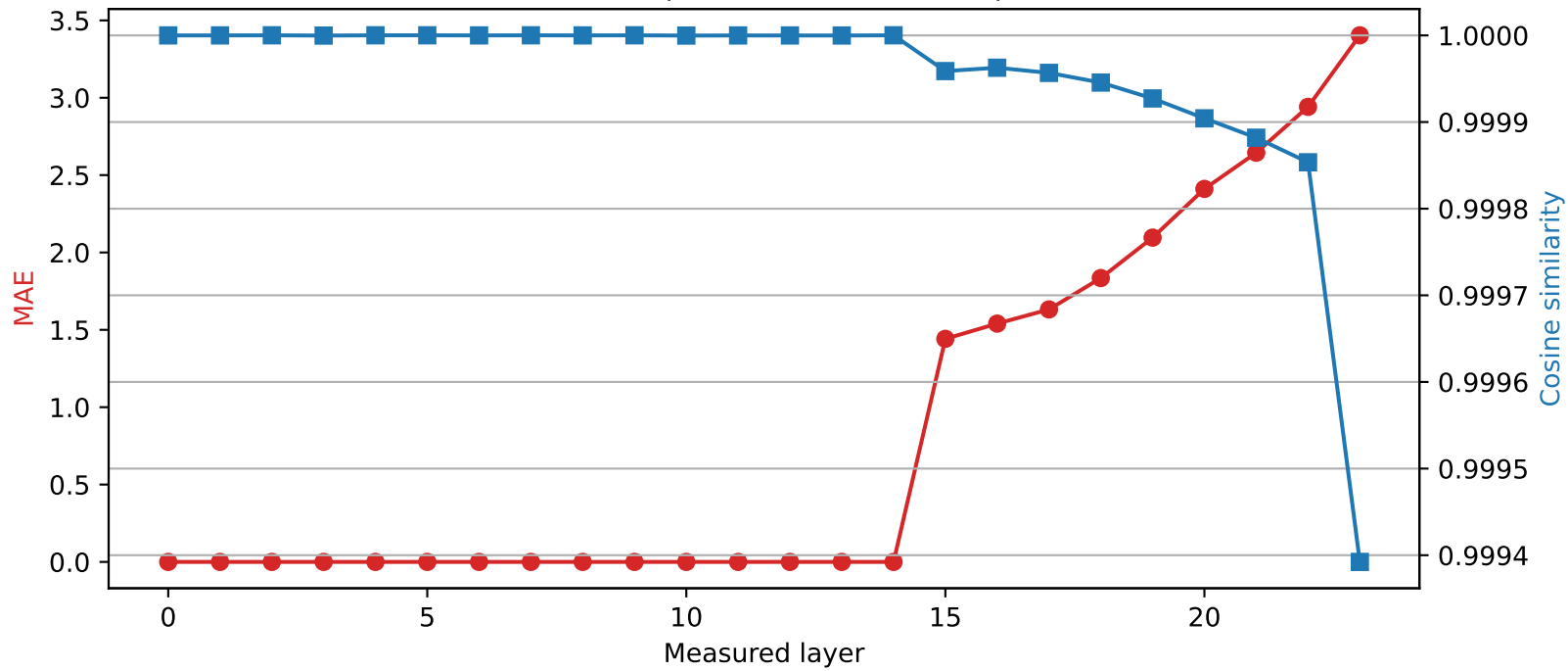
SmolLM2-1.7B-Instruct | Quantized layer 14 | float16 → int4
