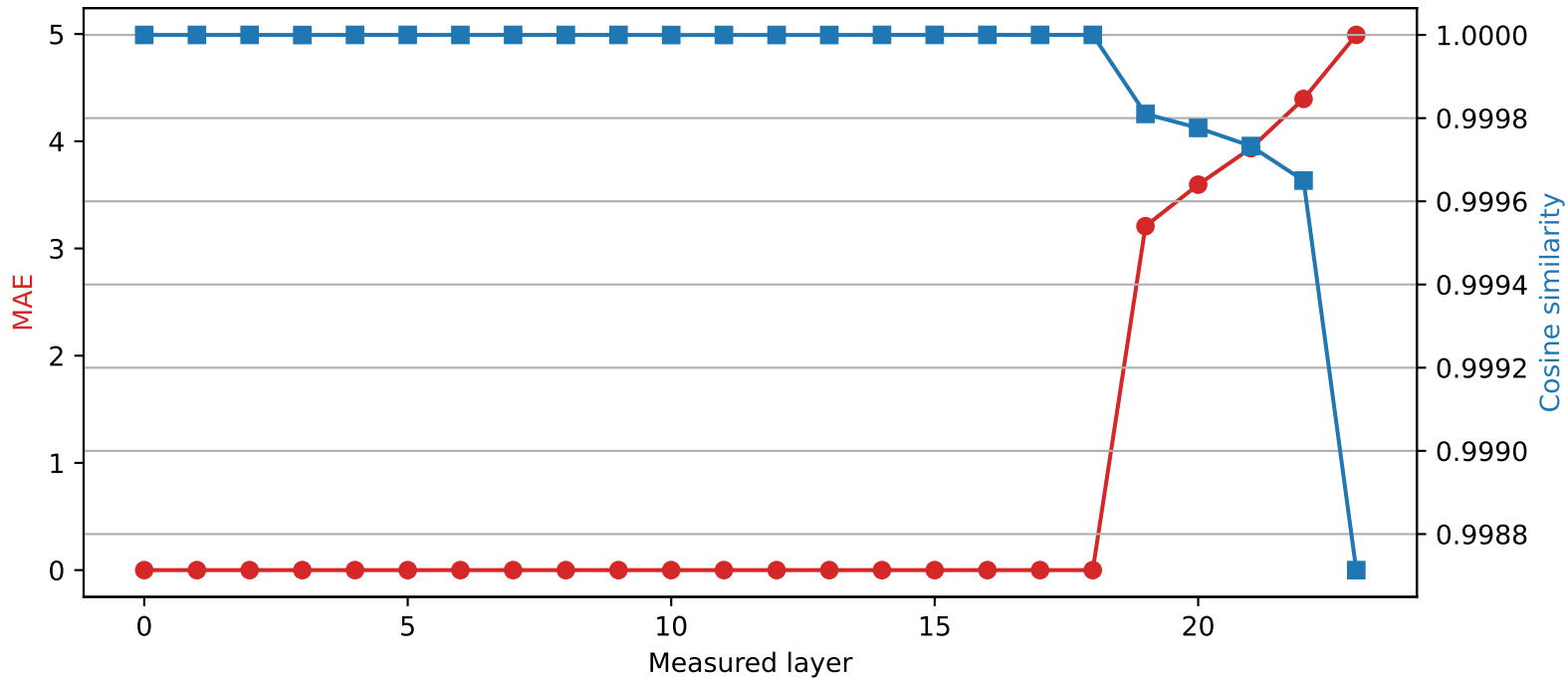
SmolLM2-1.7B-Instruct | Quantized layer 18 | float16 → int4
