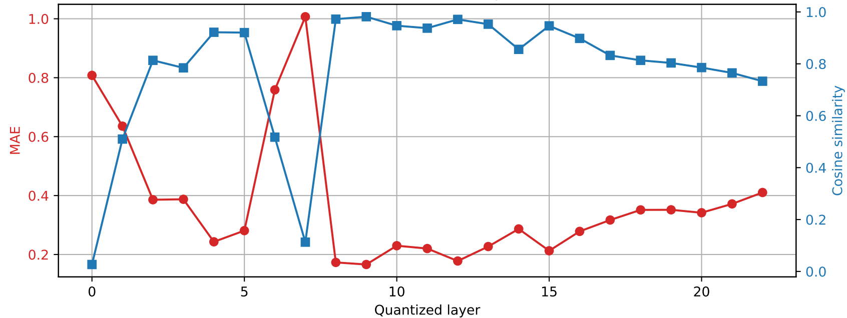
SmolLM2-1.7B-Instruct | Prompt 0 Final RMSNorm output damage | float16 \rightarrow int2
