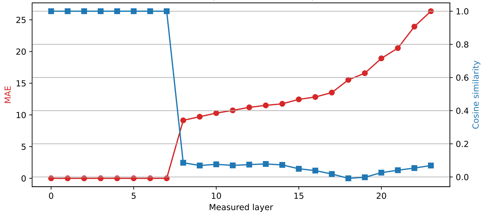
SmolLM2-1.7B-Instruct | Quantized layer 7 | float16 \rightarrow int2
