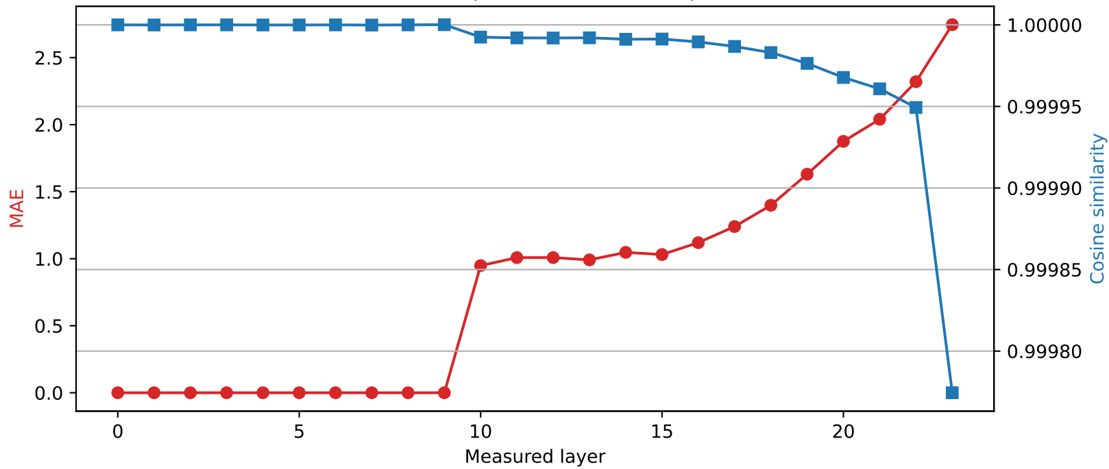
SmolLM2-1.7B-Instruct | Quantized layer 9 | float16 \rightarrow int2
