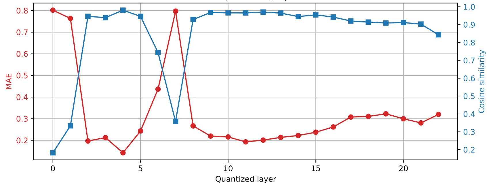
SmolLM2-1.7B-Instruct | Prompt 1 Final RMSNorm output damage | float16 \rightarrow int2
