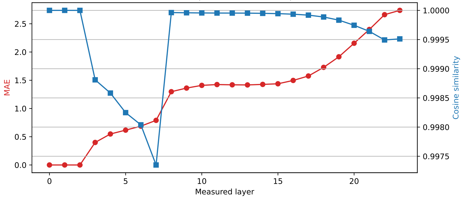
SmolLM2-1.7B-Instruct | Quantized layer 2 | float16 \rightarrow int2
