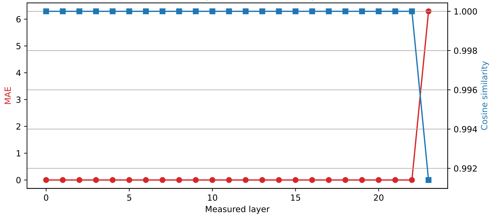
SmolLM2-1.7B-Instruct | Quantized layer 22 | float16 \rightarrow int2
