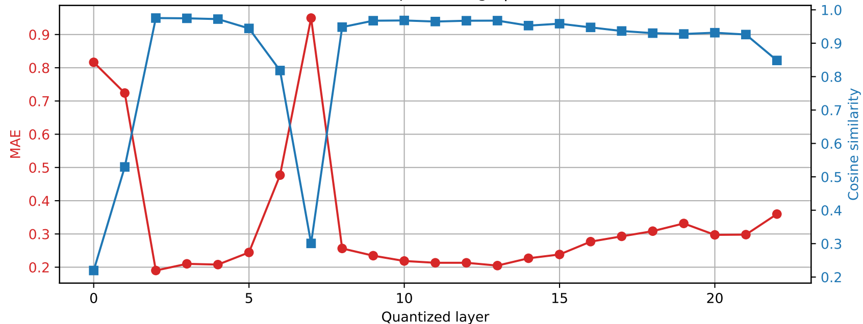
SmolLM2-1.7B-Instruct | Prompt 3 Final RMSNorm output damage | float16 \rightarrow int2
