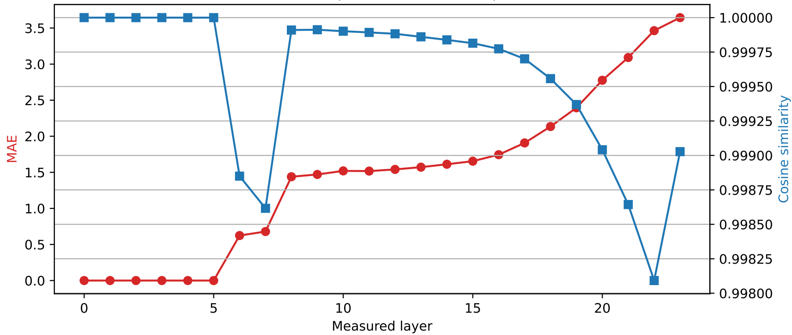
SmolLM2-1.7B-Instruct | Quantized layer 5 | float16 → int2
