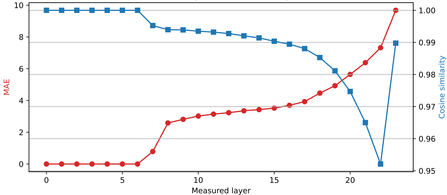
SmolLM2-1.7B-Instruct | Quantized layer 6 | float16 \rightarrow int2
