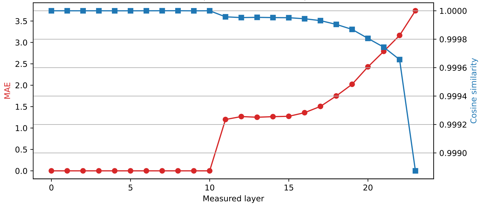
SmolLM2-1.7B-Instruct | Quantized layer 10 | float16 → int2
