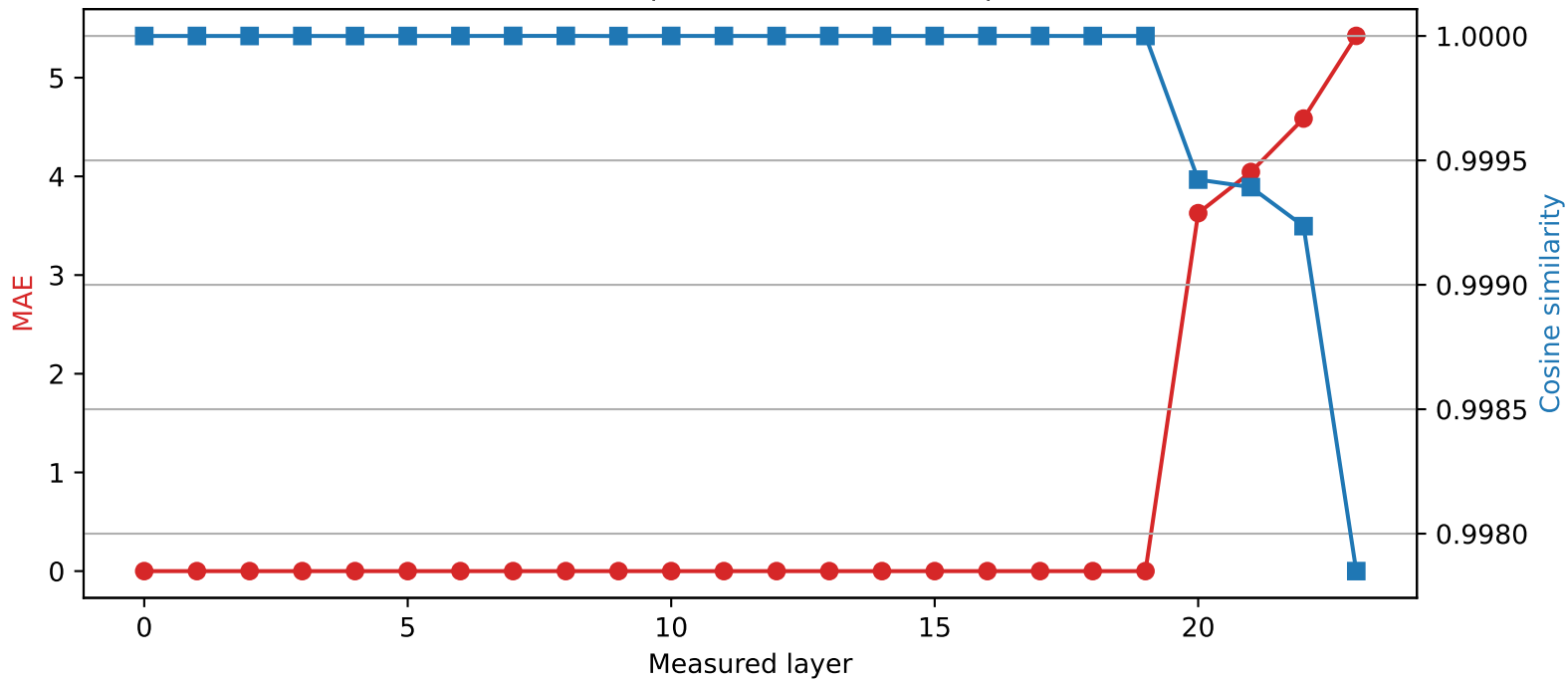
SmolLM2-1.7B-Instruct | Quantized layer 19 | float16 → int2
