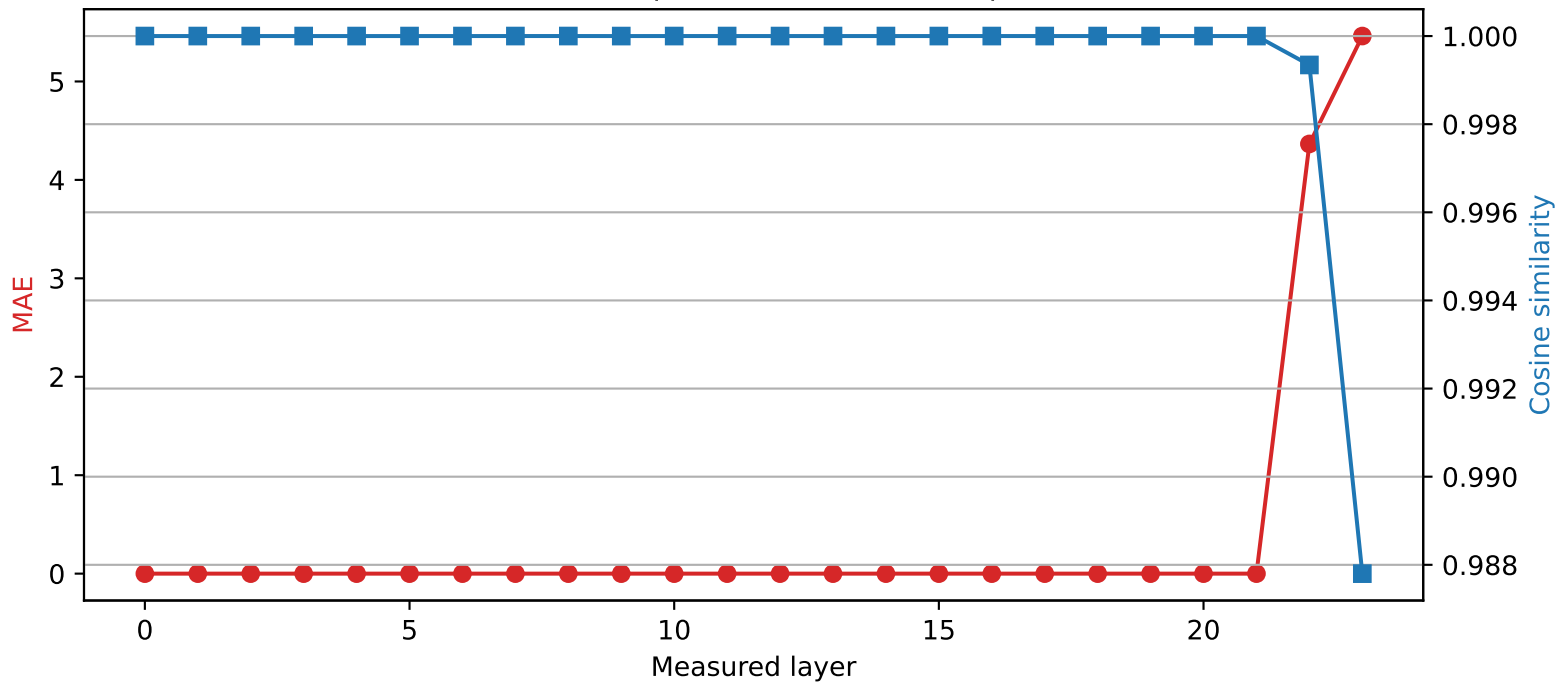
SmolLM2-1.7B-Instruct | Quantized layer 21 | float16 \rightarrow int2
