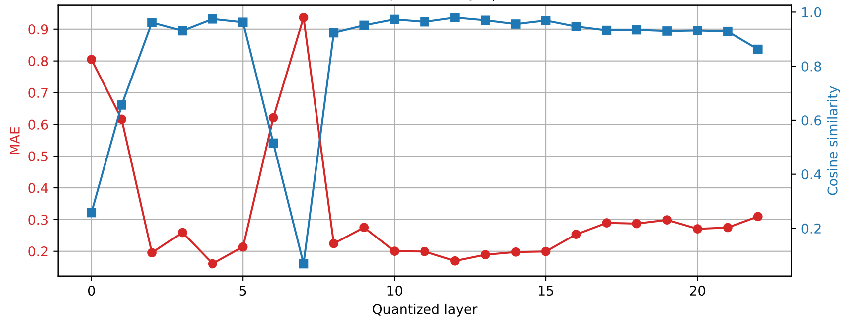
SmolLM2-1.7B-Instruct | Prompt 4 Final RMSNorm output damage | float16 \rightarrow int2
