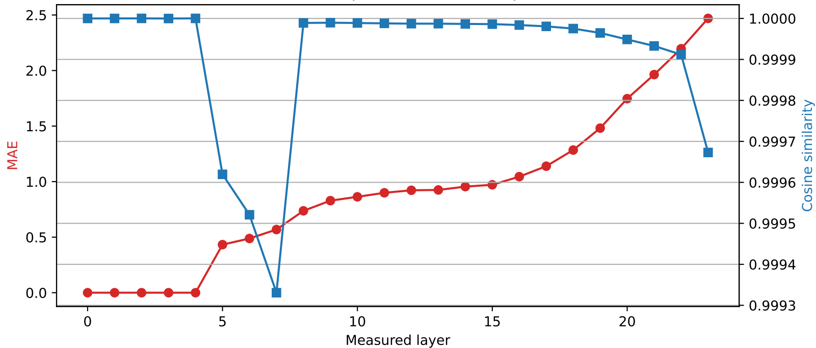
SmolLM2-1.7B-Instruct | Quantized layer 4 | float16 → int2
