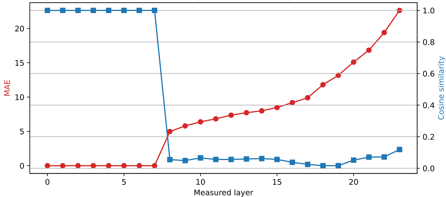
SmolLM2-1.7B-Instruct | Quantized layer 7 | float16 → int2
