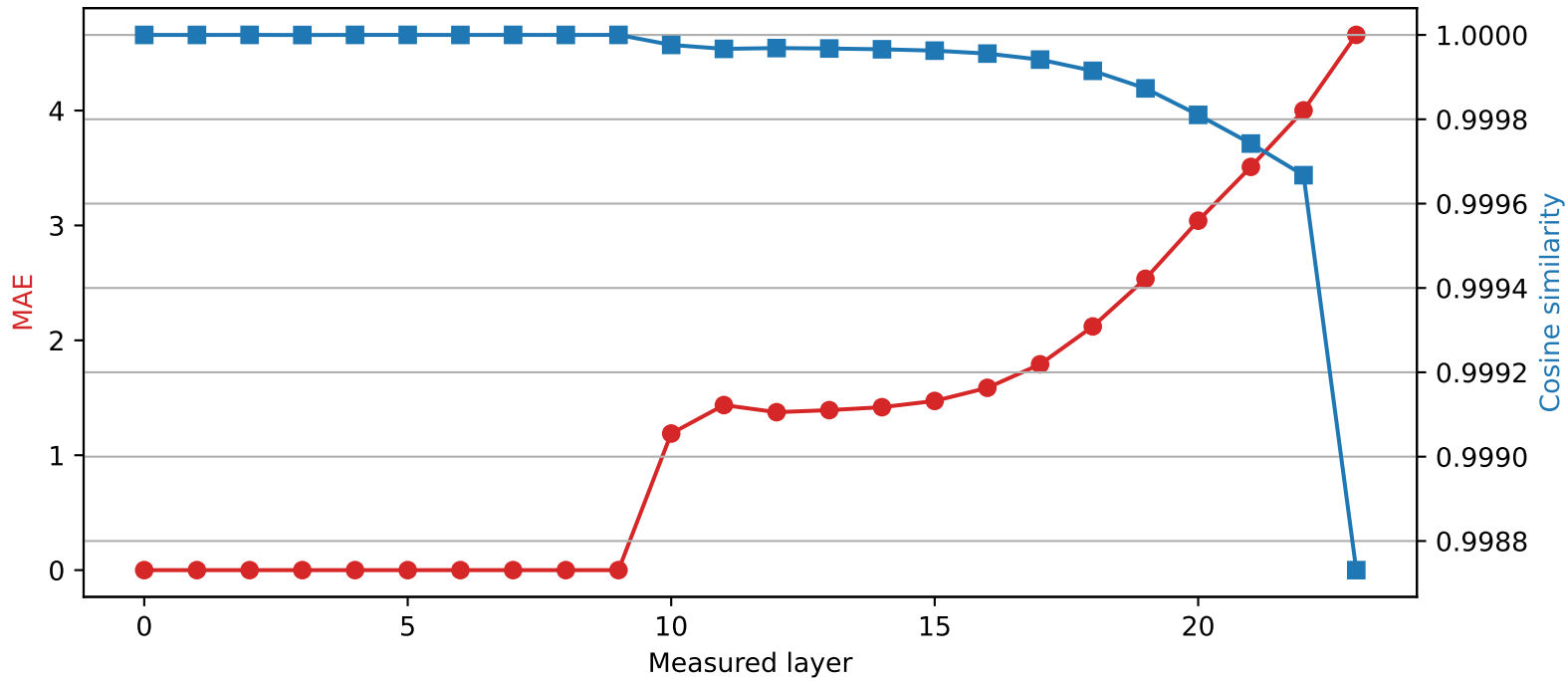
SmolLM2-1.7B-Instruct | Quantized layer 9 | float16 → int2
