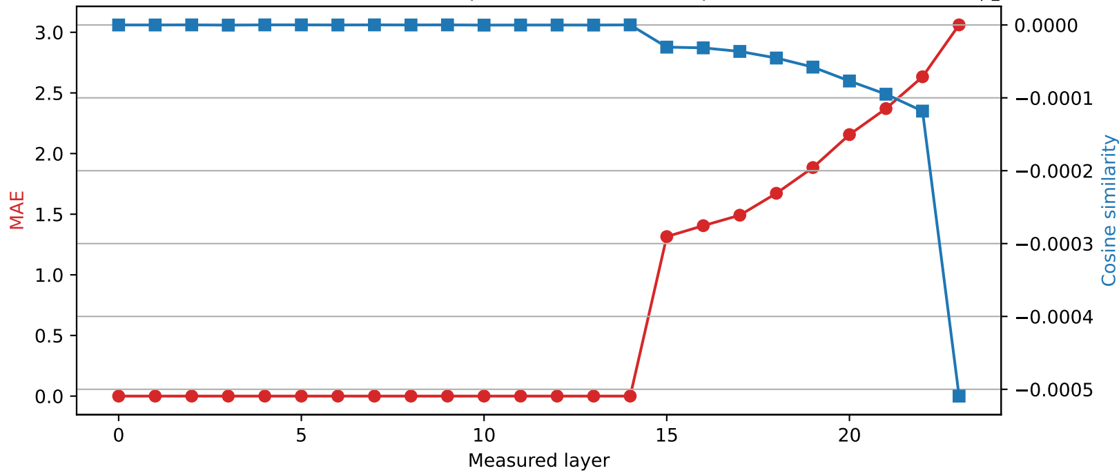
SmolLM2-1.7B-Instruct | Quantized layer 14 | float16 \rightarrow int2
