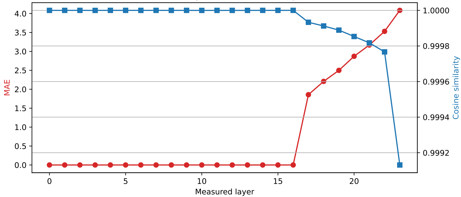
SmolLM2-1.7B-Instruct | Quantized layer 16 | float16 \rightarrow int2
