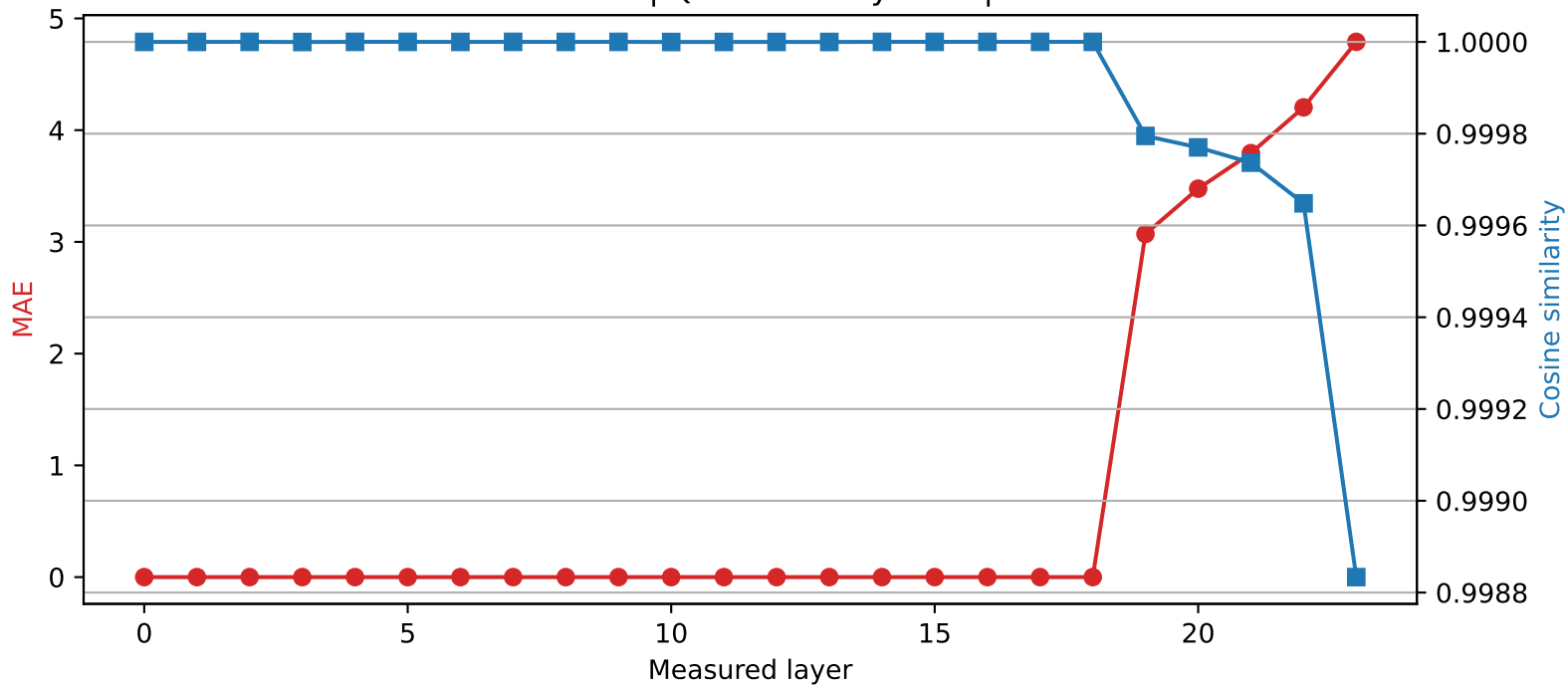
SmolLM2-1.7B-Instruct | Quantized layer 18 | float16 → int2
