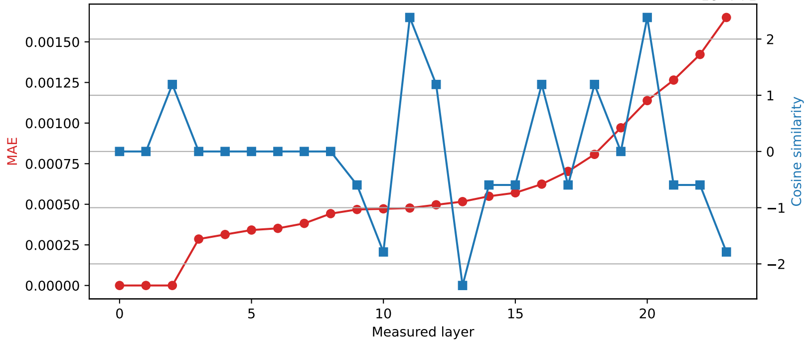
SmolLM2-1.7B-Instruct | Quantized layer 2 | float32 → int16
