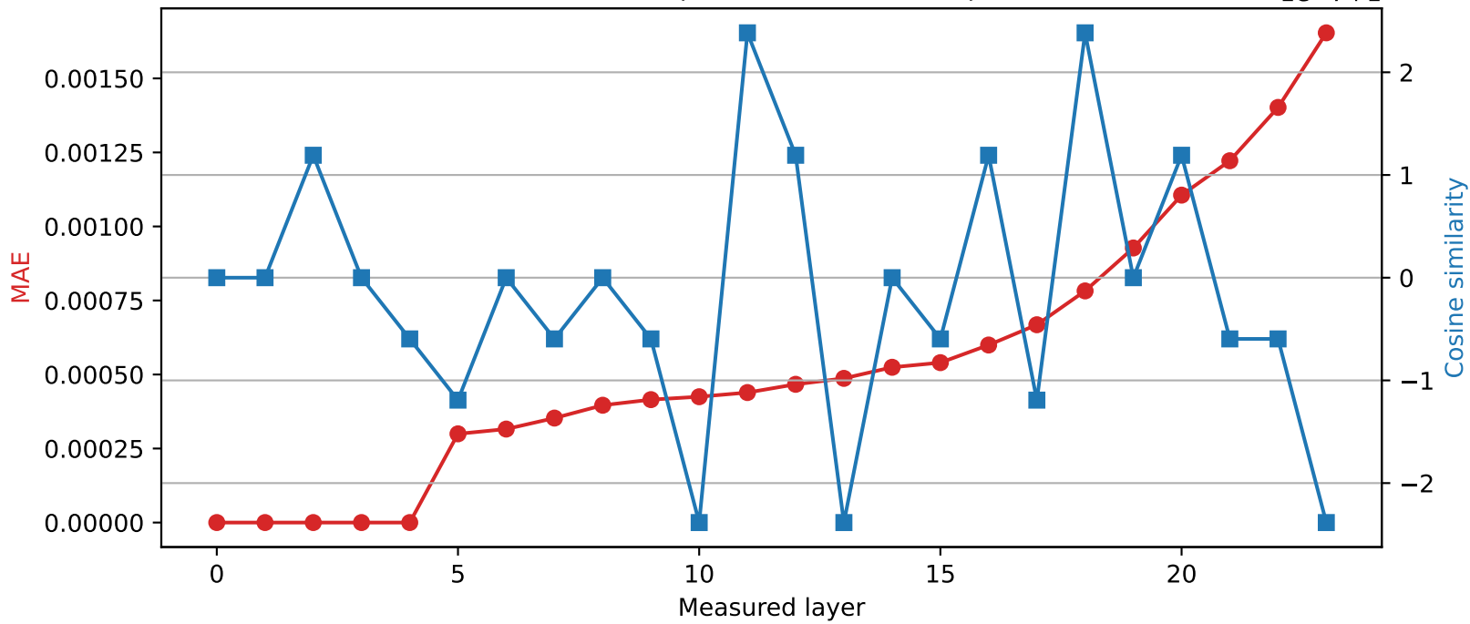
SmolLM2-1.7B-Instruct | Quantized layer 4 | float32 \rightarrow int16
