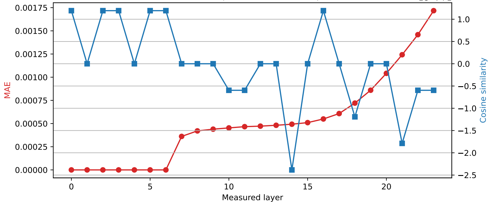
SmolLM2-1.7B-Instruct | Quantized layer 6 | float32 \rightarrow int16
