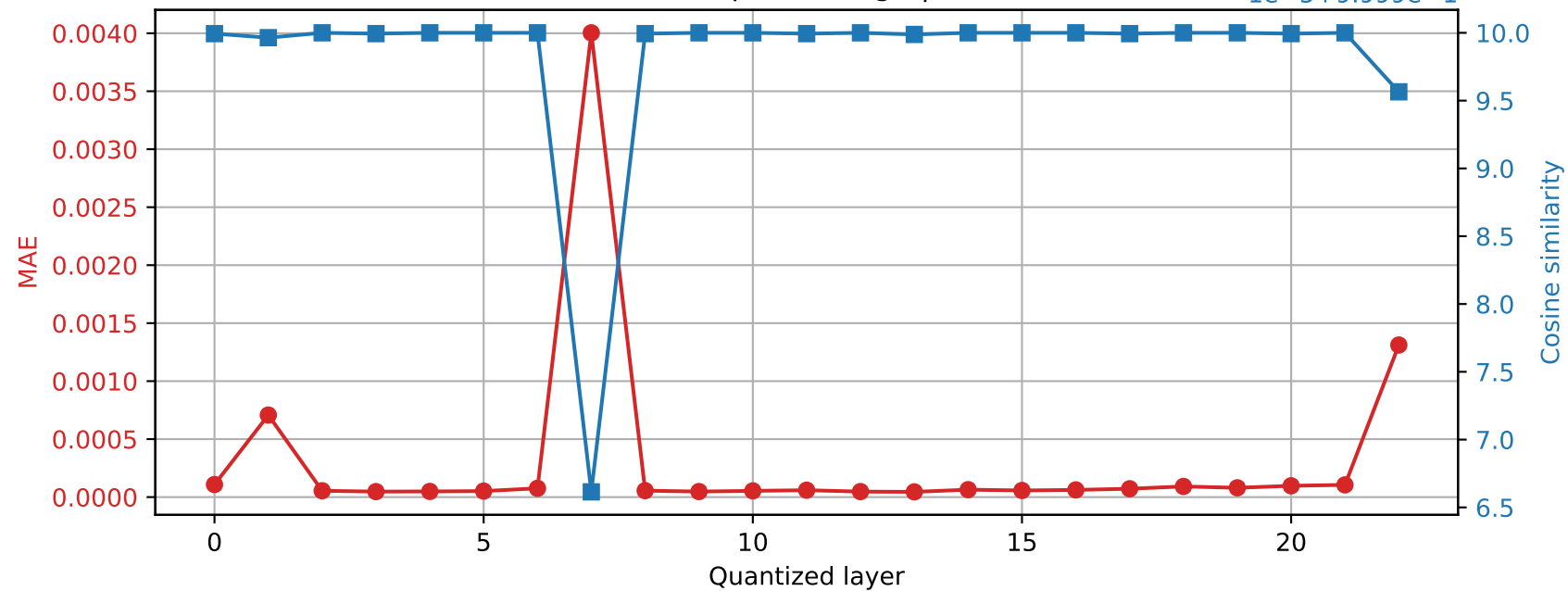
SmolLM2-1.7B-Instruct | Prompt 2 Final RMSNorm output damage | float32 → int16
