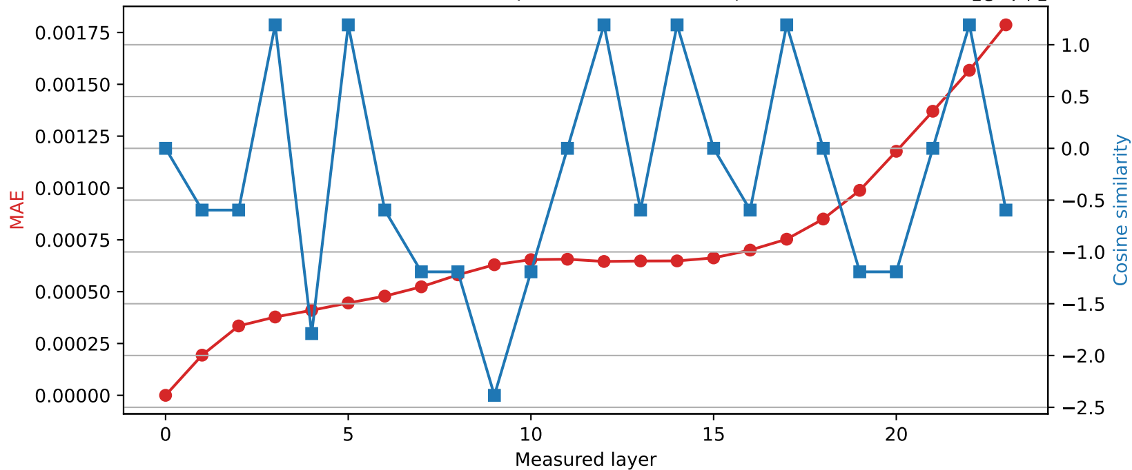
SmolLM2-1.7B-Instruct | Quantized layer 0 | float32 \rightarrow int16
