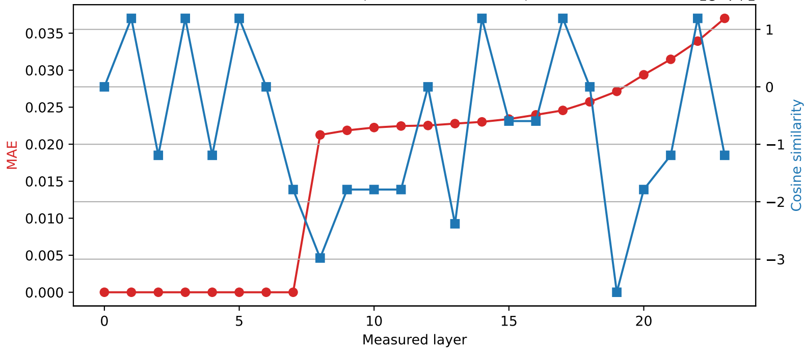
SmolLM2-1.7B-Instruct | Quantized layer 7 | float32 \rightarrow int16
