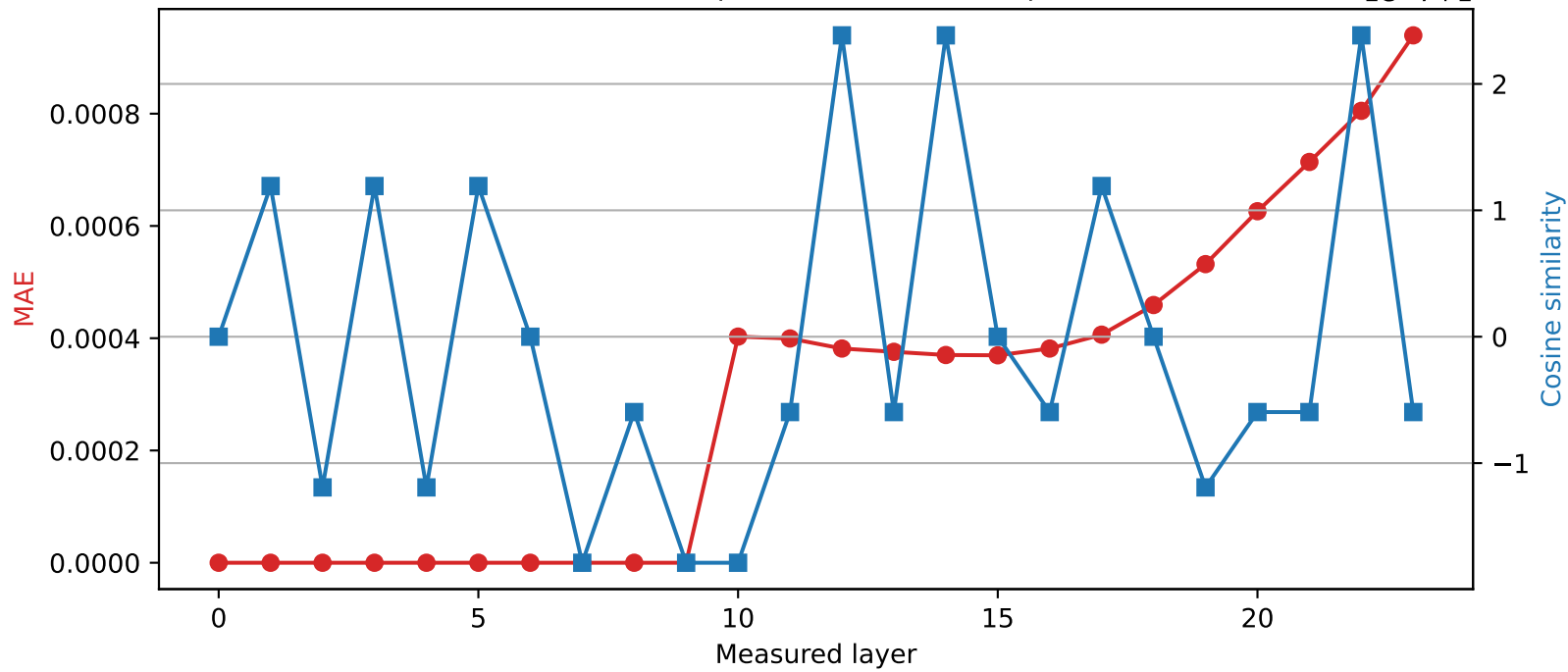
SmolLM2-1.7B-Instruct | Quantized layer 9 | float32 \rightarrow int16
