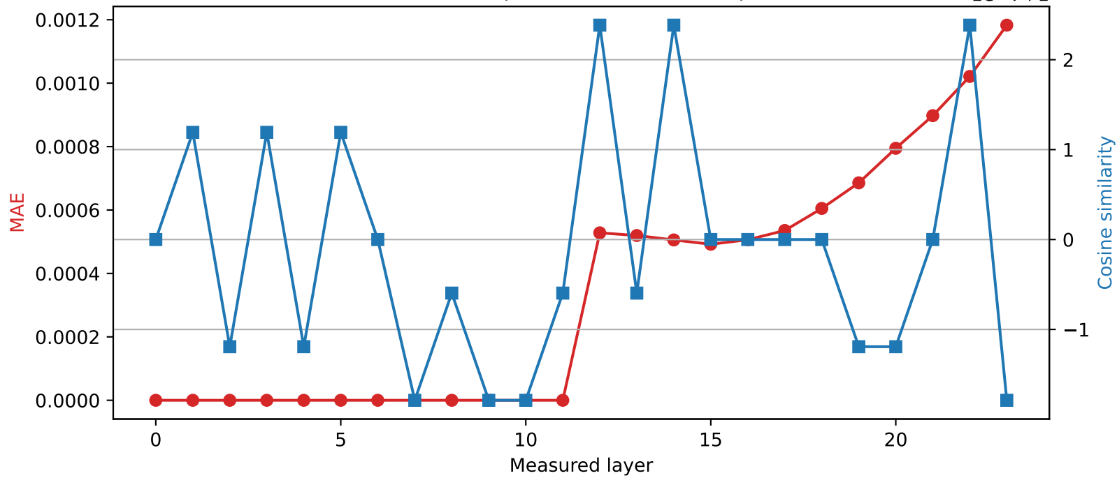
SmolLM2-1.7B-Instruct | Quantized layer 11 | float32 \rightarrow int16
