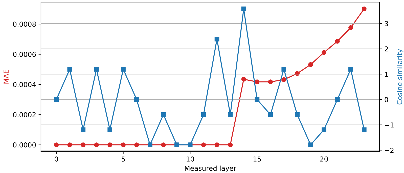
SmolLM2-1.7B-Instruct | Quantized layer 13 | float32 \rightarrow int16
