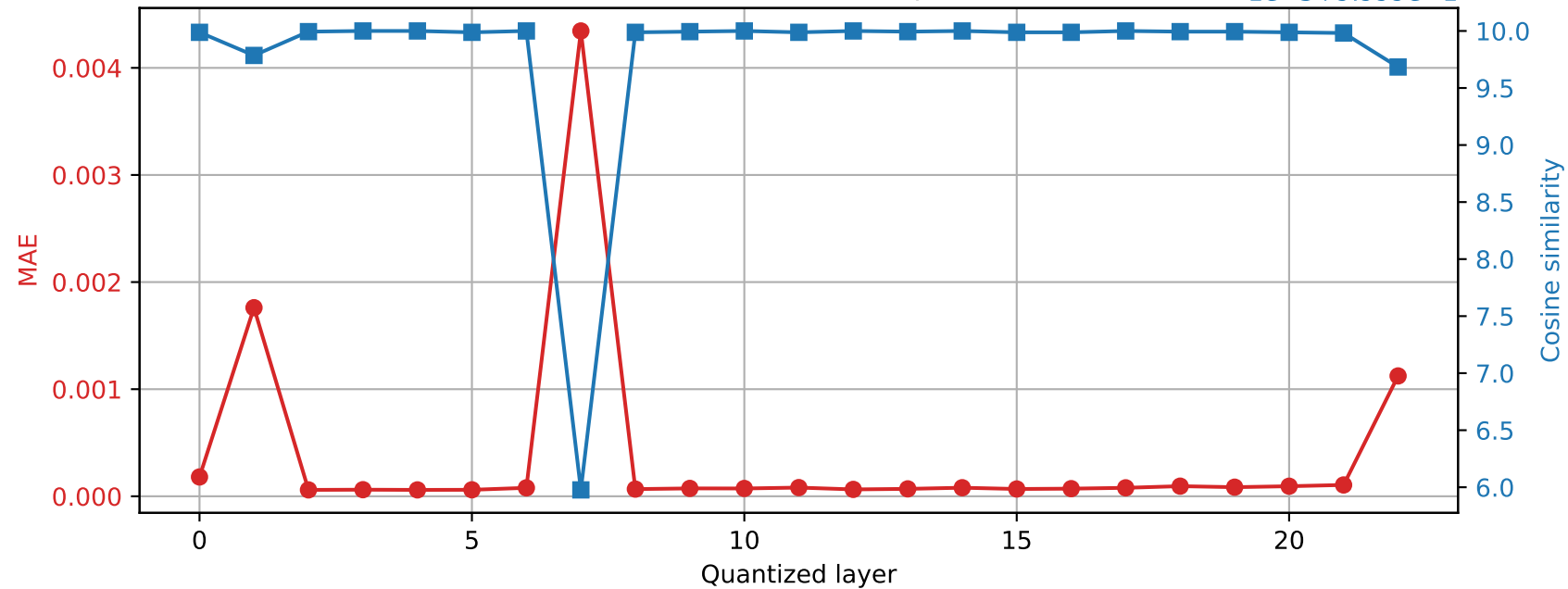
SmolLM2-1.7B-Instruct | Prompt 3 Final RMSNorm output damage | float32 \rightarrow int16
