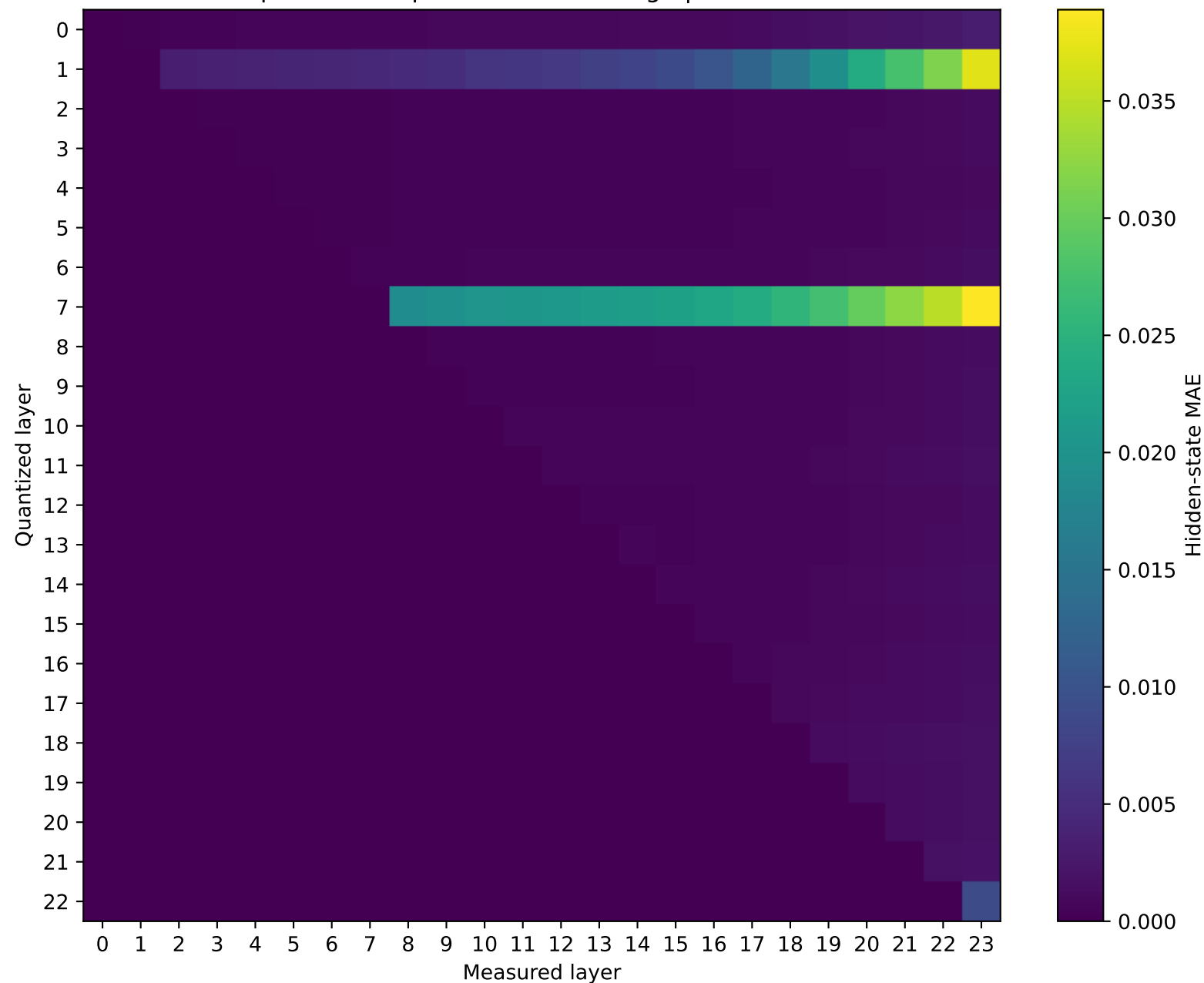
SmolLM2-1.7B-Instruct Prompt 3: MAE representation damage | float32 → int16
