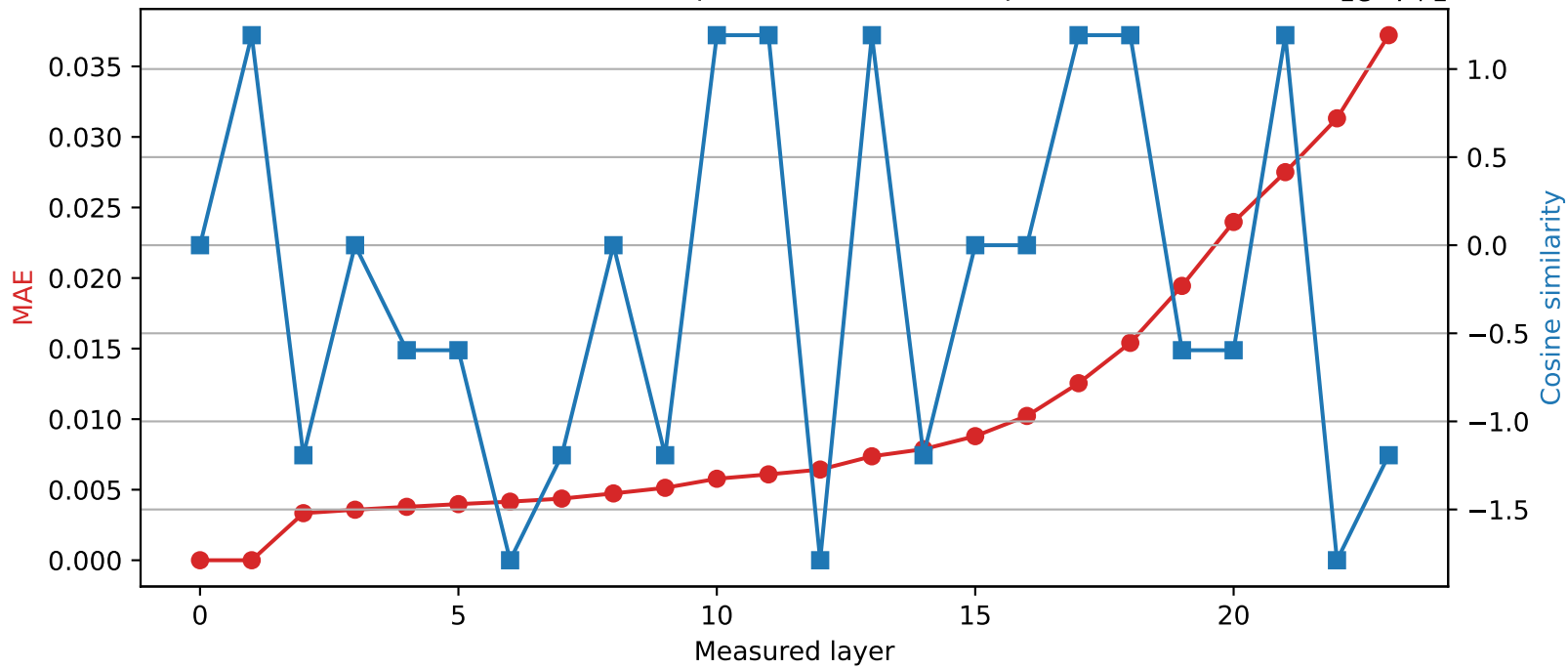
SmolLM2-1.7B-Instruct | Quantized layer 1 | float32 \rightarrow int16
