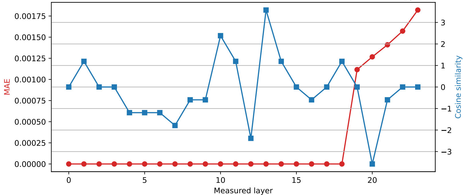
SmolLM2-1.7B-Instruct | Quantized layer 18 | float32 \rightarrow int16
